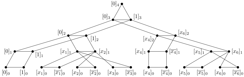
Fig. 3. The graph representation G_L of the normal form N_L considered in Example 5.11. The levels are omitted from the vertex names as they are clear from the graph structure.
