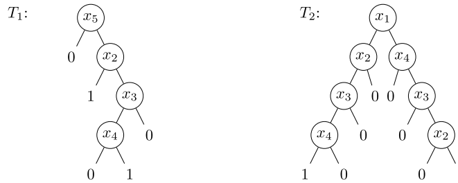
Fig. 1. The decision tree T_1 computes the function x_5 \wedge (\bar{x}_2 \vee \bar{x}_3 \wedge x_4) and has rank 1. The decision tree T_2 computes the function x_1 \wedge x_2 \wedge x_3 \wedge x_4 \vee \bar{x}_1 \wedge \bar{x}_2 \wedge \bar{x}_3 \wedge \bar{x}_4 and has rank 2.
