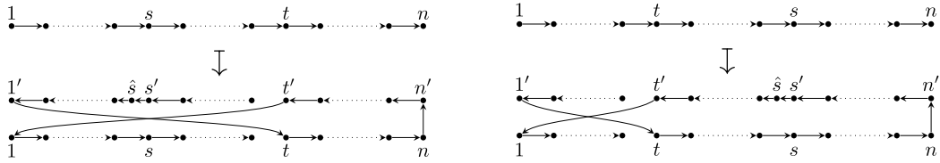
Fig. 2. The reduction from ORD to DiPATHCENTER.
