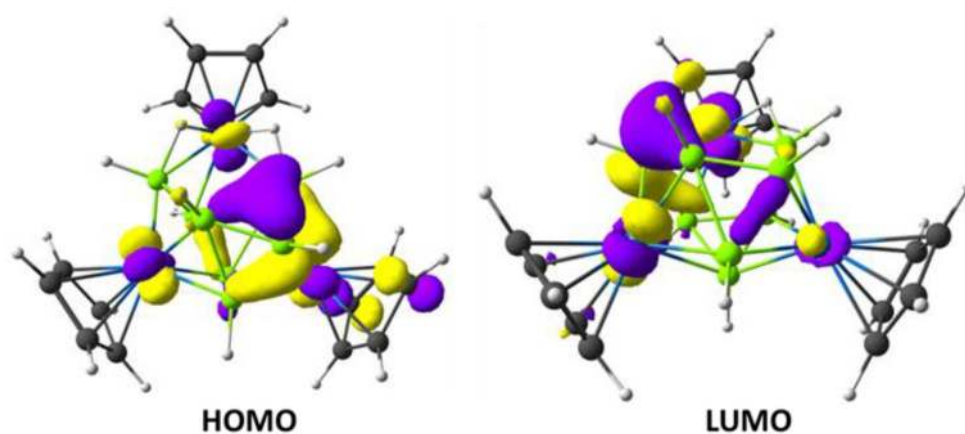
Figure 4. Frontier molecular orbitals of 1' . Contour value: \pm 0.05 [\text{e}/\text{bohr}^3]^{1/2} .
