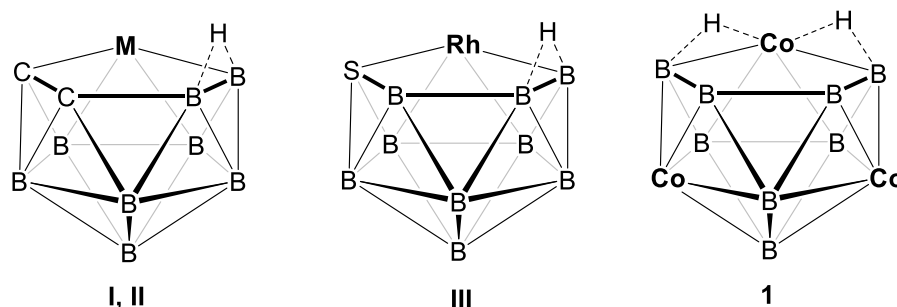
I: M = \text{Ir}(\text{PPh}_3)_2 ; II: M = \text{Rh}(\text{PEt}_3)_2 ; III: \text{Rh} = \text{Rh}(\text{PPh}_3)_2 , Co = \text{Cp}^*\text{Co} ; C = \text{CH} ; B = \text{BH}
