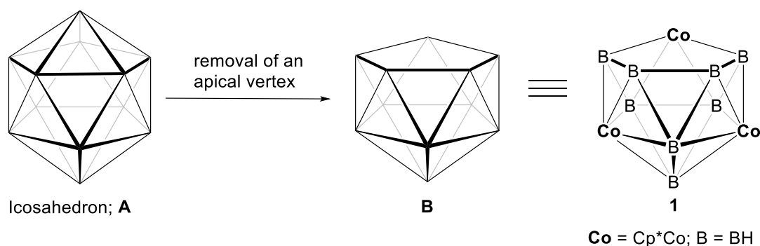
Figure 2. Schematic representation of stepwise generation of the cluster framework of 1 (B) from an icosahedron (A).
