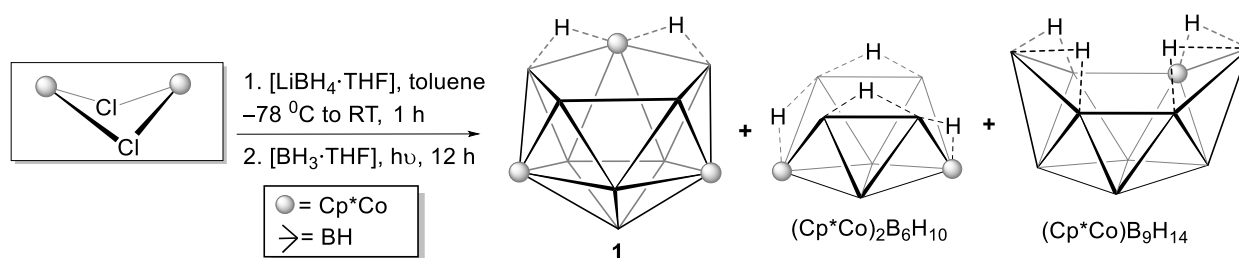
Scheme 1. Synthesis of the open-faced tricobaltaborane cluster 1 .
