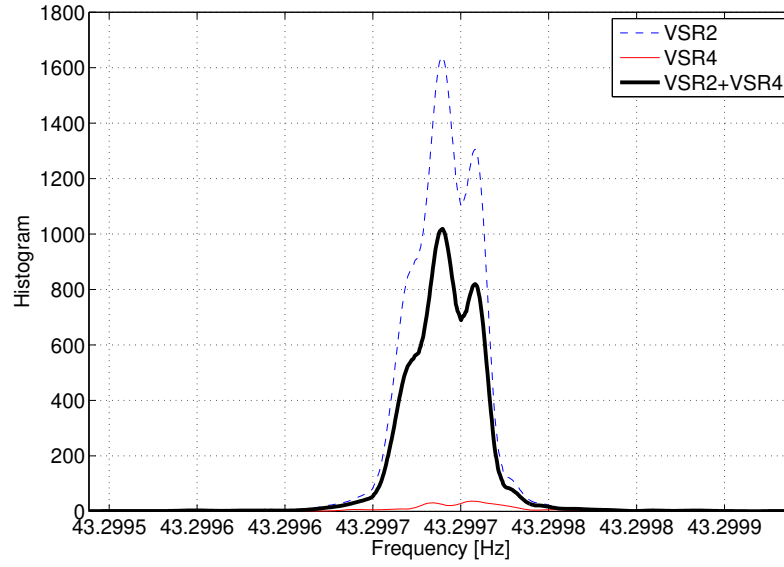
FIG. 16. Final peakmap histograms for the outliers at 43.30 Hz. The dark thick curve corresponds to the full VSR2/VSR4 analysis; the light continuous (red in color version) curve corresponds to VSR4 analysis while the light dashed (blue in color version) curve corresponds to the analysis of VSR2 alone.
